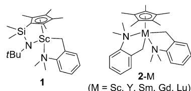
Figure 1. Half-sandwich rare-earth mono- and dialkyl complexes.
